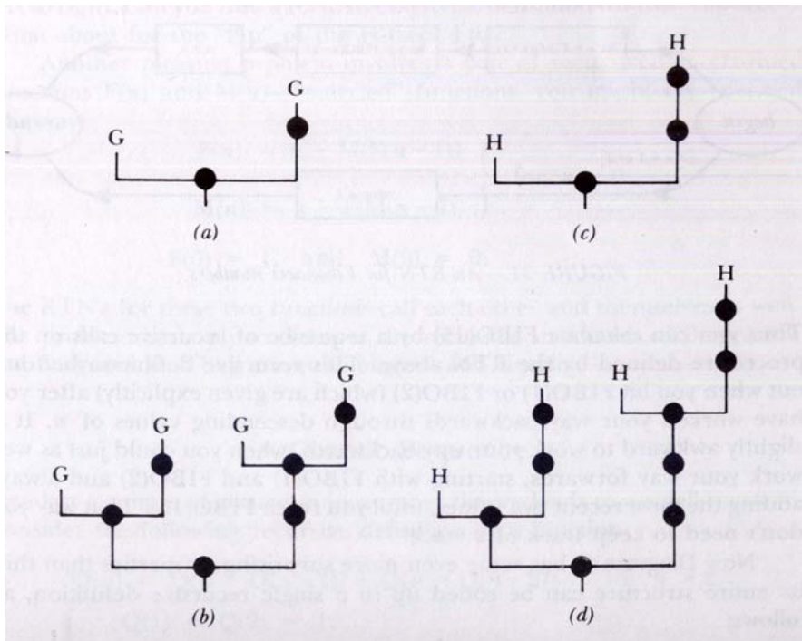
FIGURE 29. (a) Diagram G, unexpanded. (c) Diagram H, unexpanded (b) Diagram G, expanded once. (d) Diagram H, expanded once
